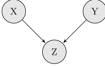
Figure 2: Common Effect Structure
