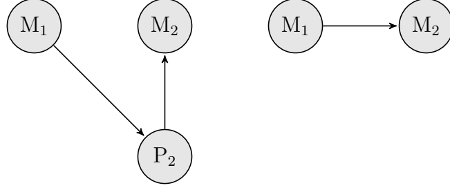
Figure 6: Minimal DAG's over \mathbf{V}_1 and \mathbf{V}_2
